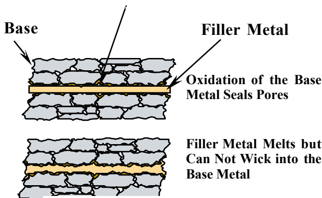
Figure 4. Effect of Oxidation on Brazing of cleanliness of stainless steel components than brazing steel components. The Chromium in the stainless steel forms a much more stable oxide at a much lower Oxygen level than Iron.
