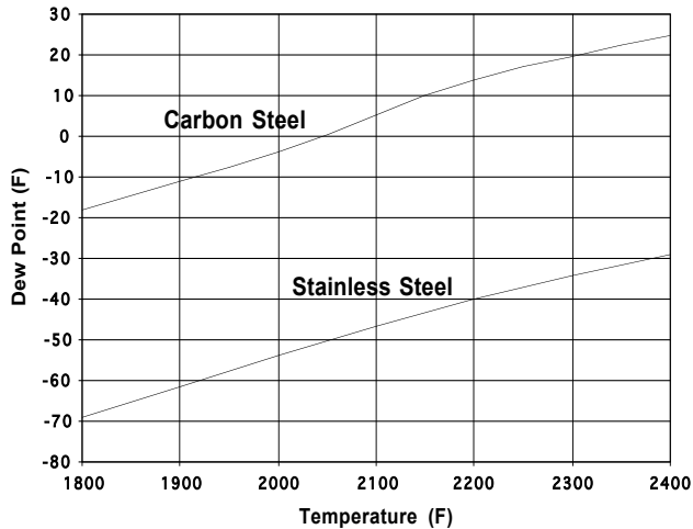
Figure 7. Dew Point Requirements
