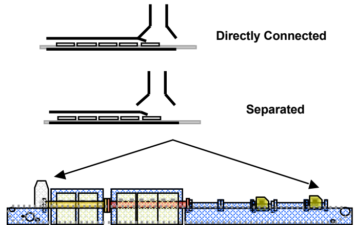
Figure 10. Furnace Stacking
