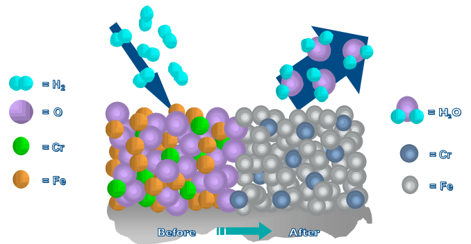
Figure 6. Oxide Reduction Mechanism
