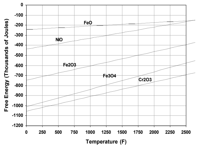
Figure 5. Oxide Stability
