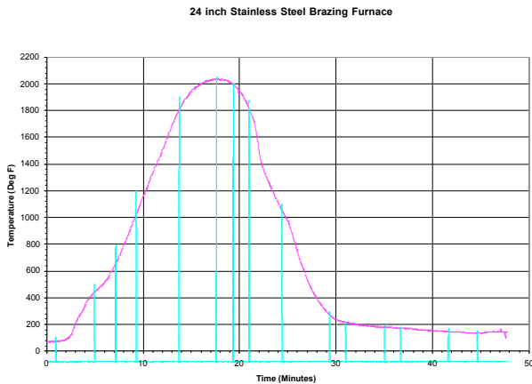
Figure 3. Example of a Temperature Profile
