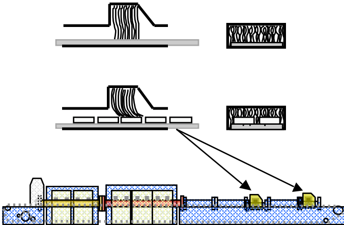
Figure 12. Schematic of Curtains and Curtain Boxes
